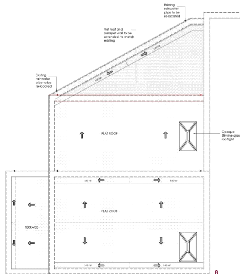
ROOF PLAN
